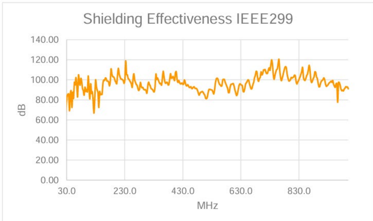
Test Position 4, 30-1000 MHz Horizontal
