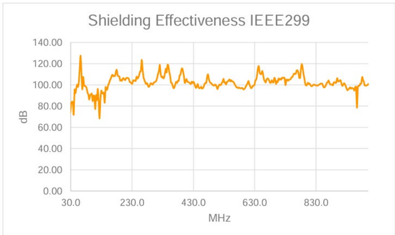
Test Position 24, 30 - 1000 MHz Horizontal
