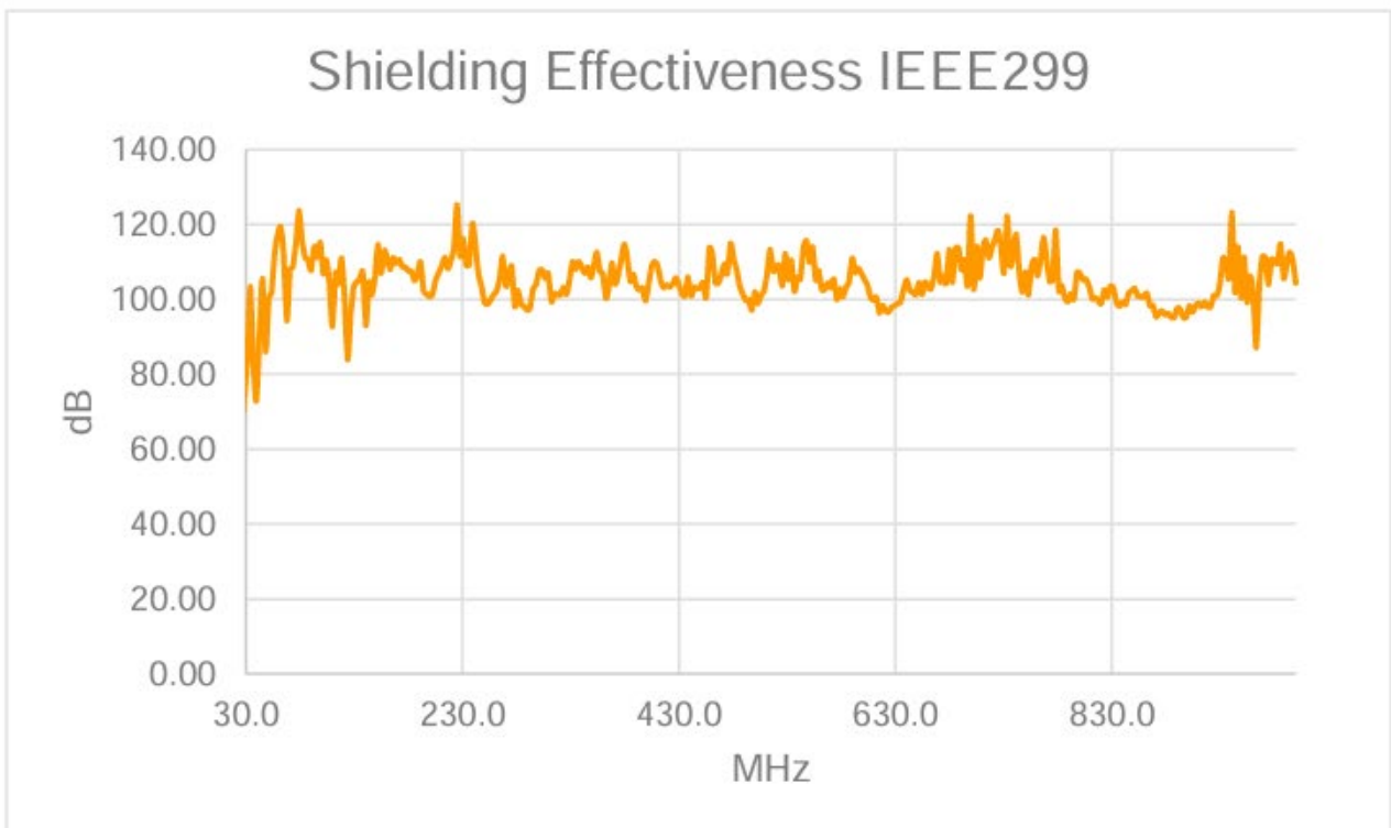
Test Position 14, 30 - 1000 MHz Horizontal
