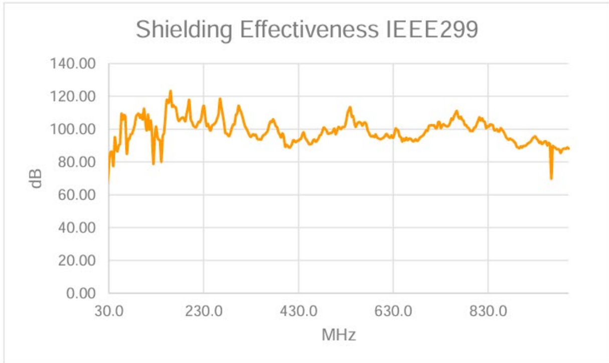
Test Position 4, 30-1000 MHz Vertical
