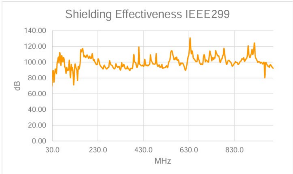
Test Position 18, 30 - 1000 MHz Horizontal
