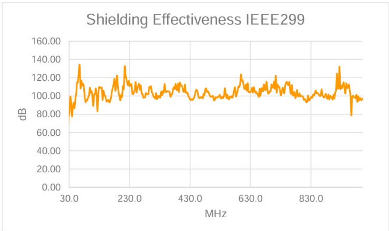
Test Position 15, 30 - 1000 MHz Horizontal
