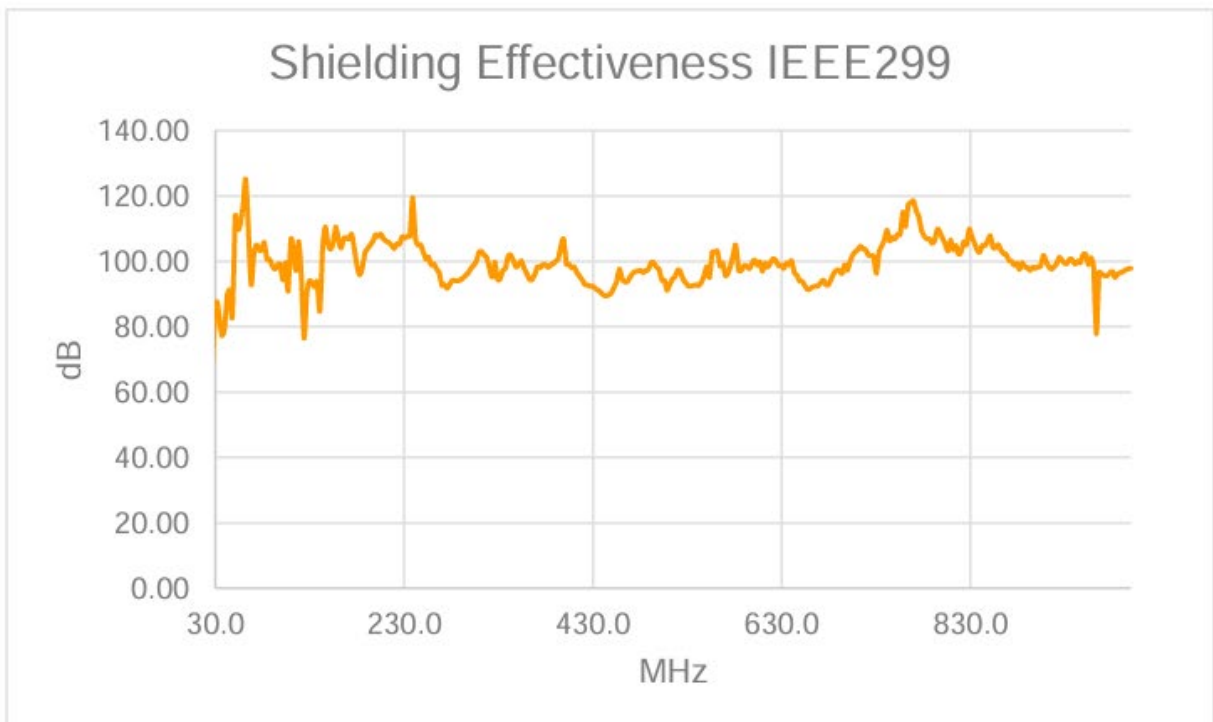
Test Position 21, 30 - 1000 MHz Horizontal
