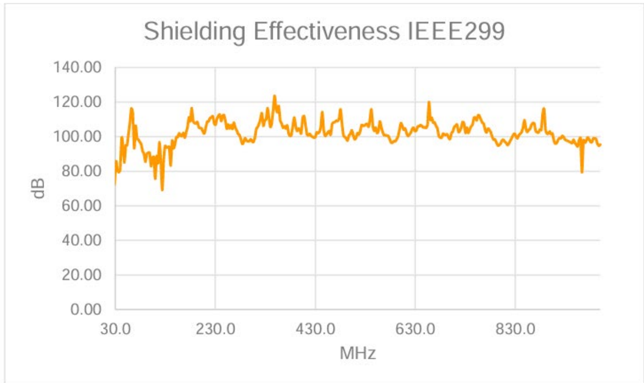
Test Position 24, 30 - 1000 MHz Vertical
