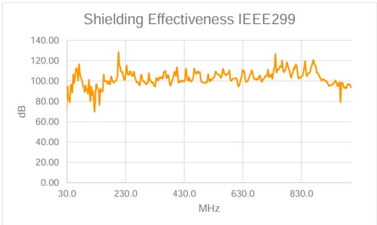
Test Position 12, 30 - 1000 MHz Horizontal
