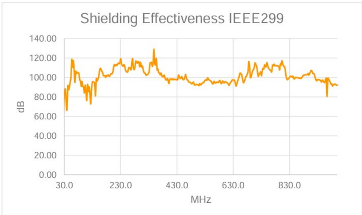
Test Position 16, 30 - 1000 MHz Horizontal
