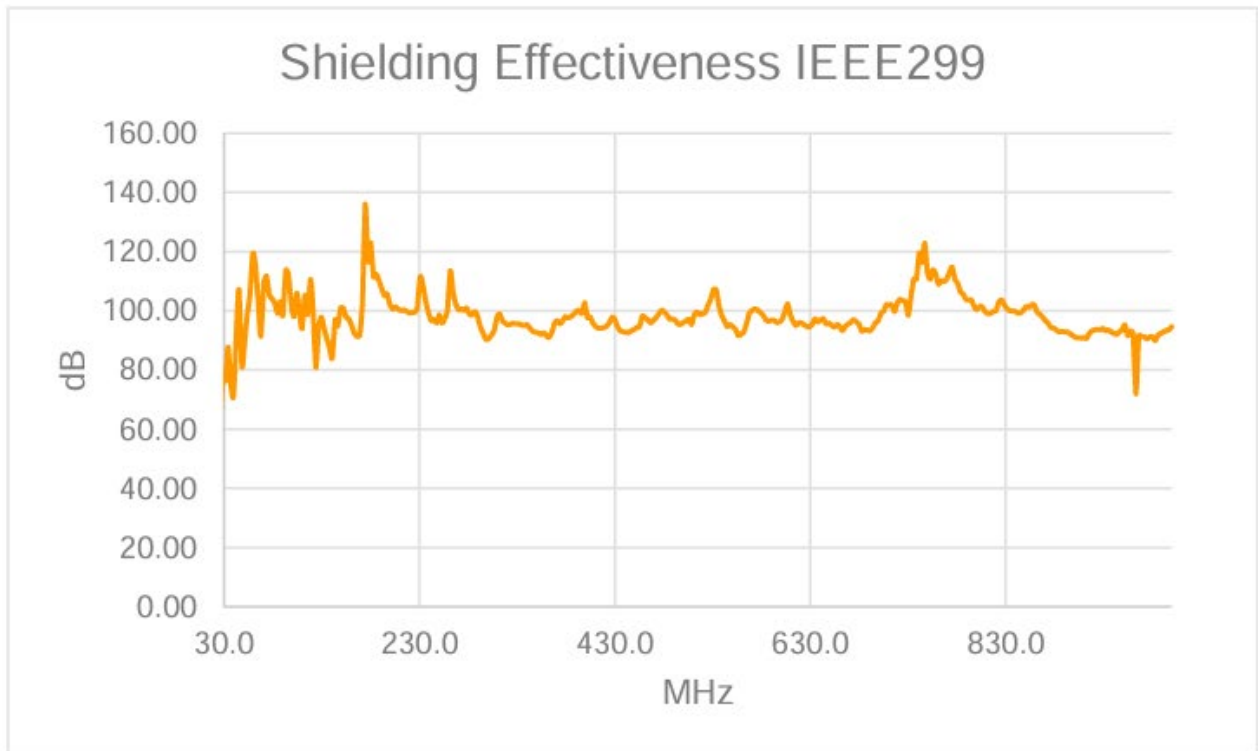
Test Position 13, 30 - 1000 MHz Vertical
