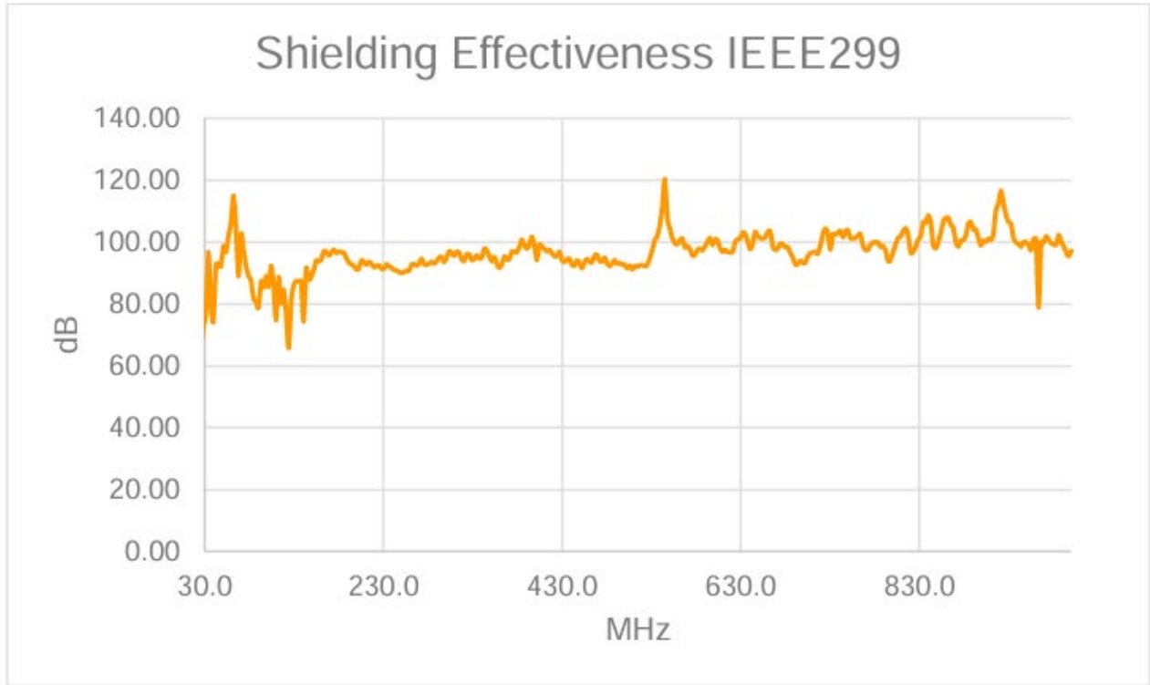
Test Position 22, 30 - 1000 MHz Vertical
