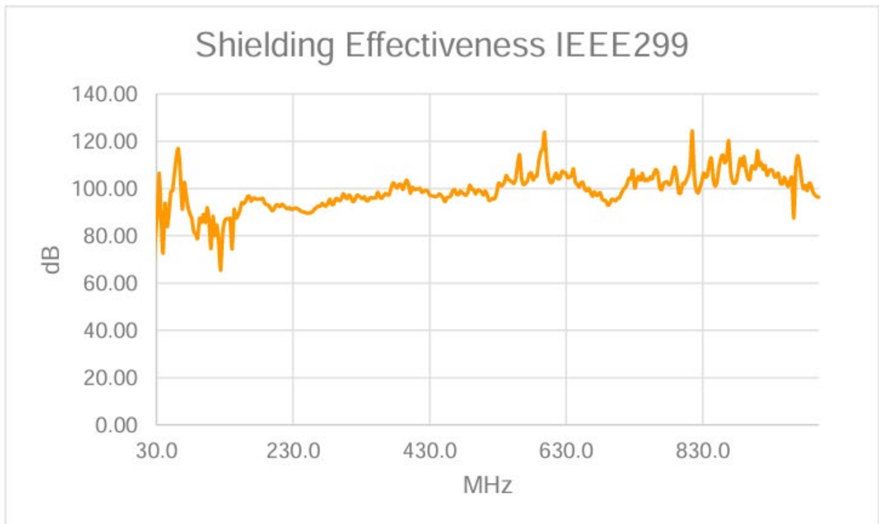
Test Position 22, 30 - 1000 MHz Horizontal
