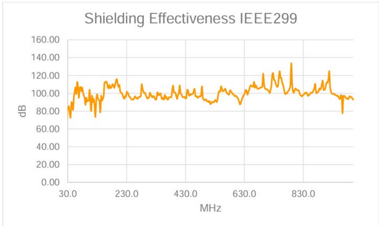
Test Position 18, 30 - 1000 MHz Vertical
