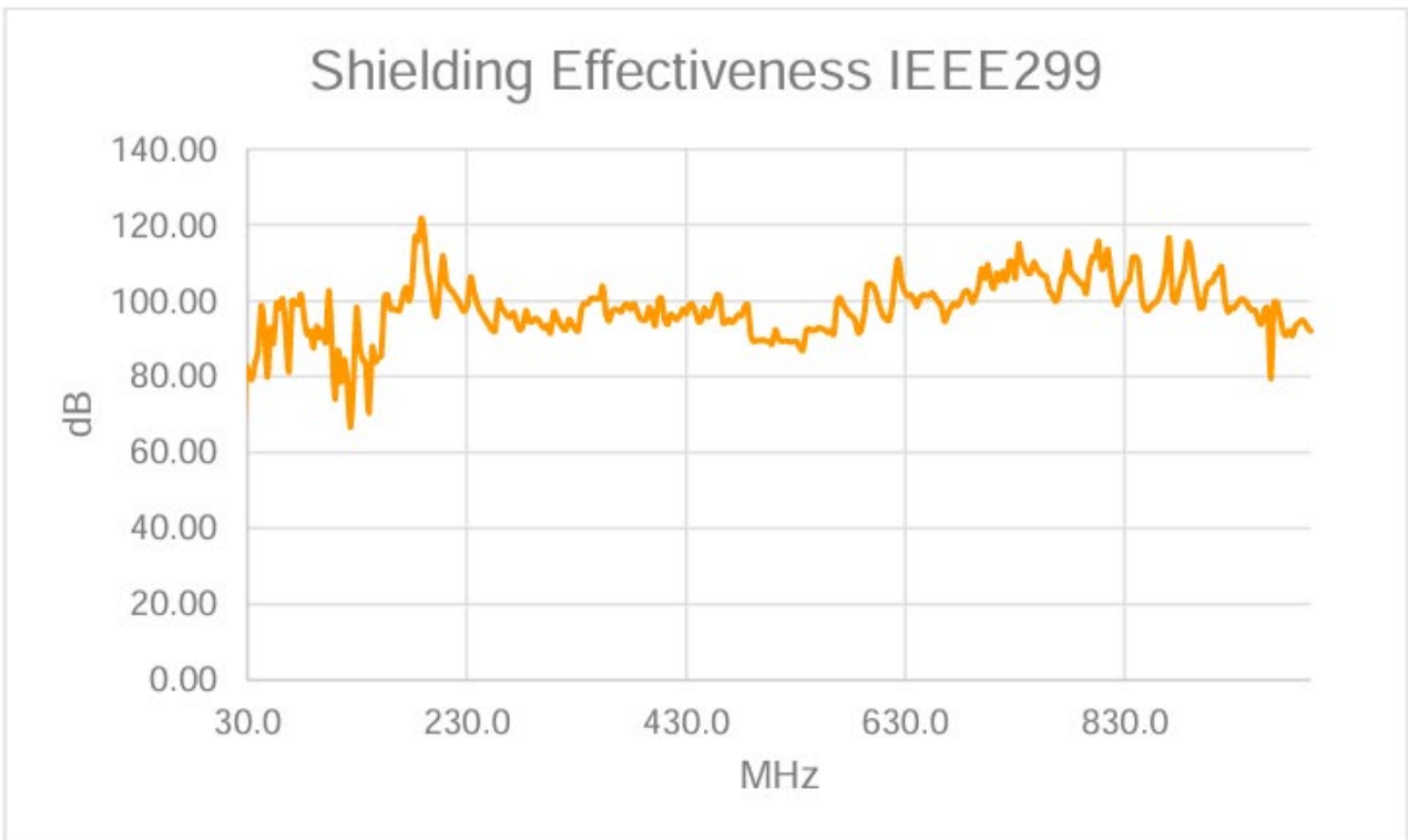
Test Position 17, 30 - 1000 MHz Horizontal
