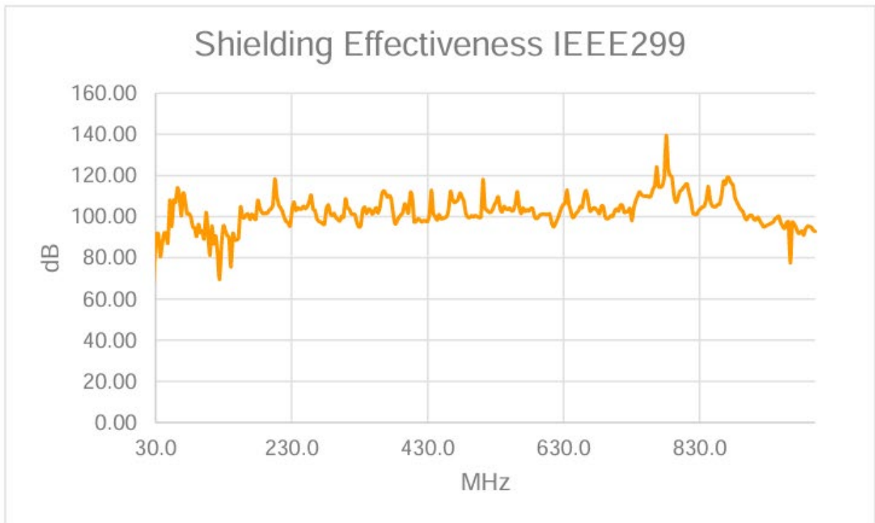
Test Position 12, 30 - 1000 MHz Vertical
