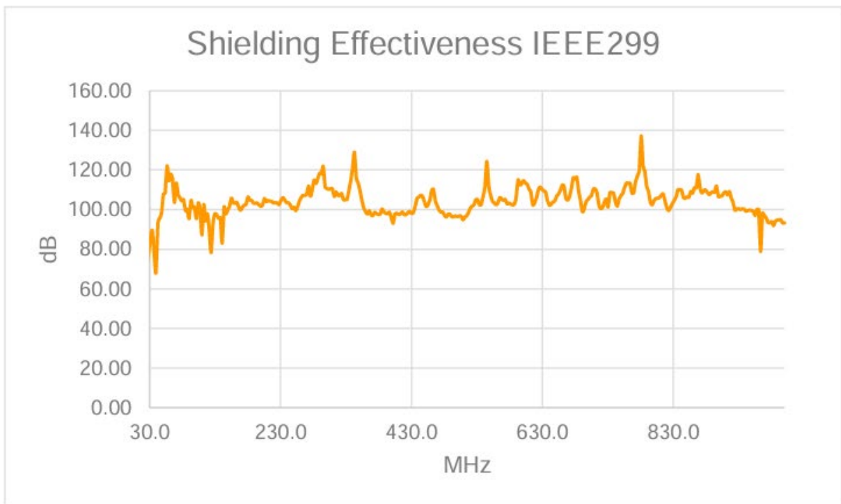
Test Position 10, 30-1000 MHz Horizontal
