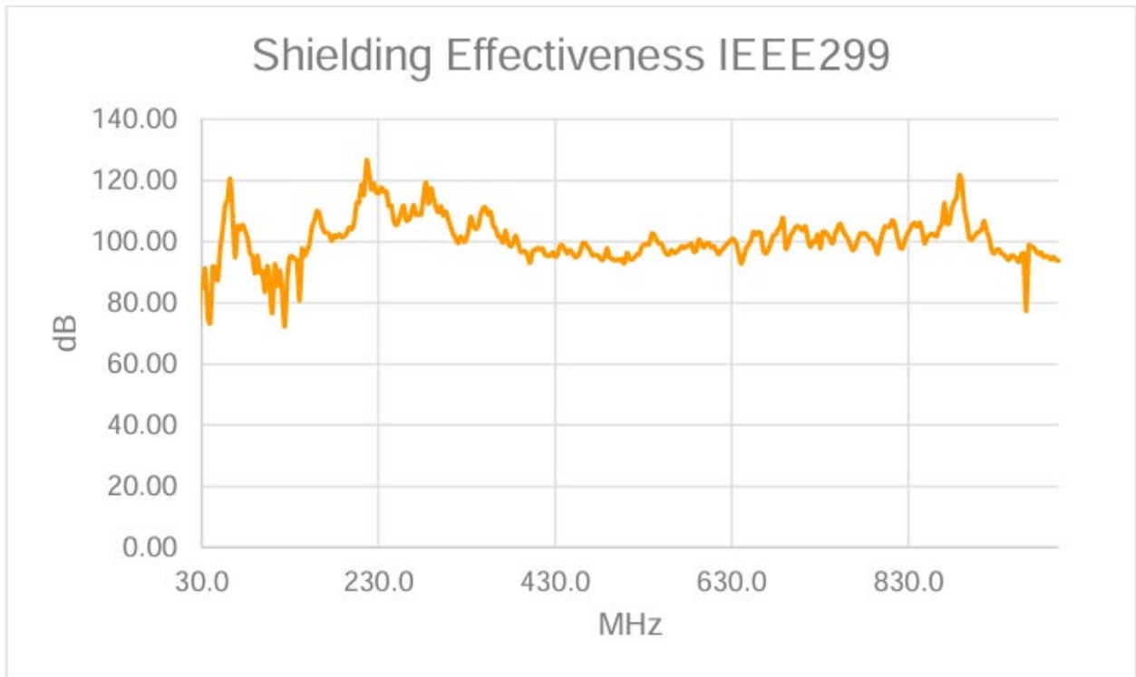
Test Position 16, 30 - 1000 MHz Vertical
