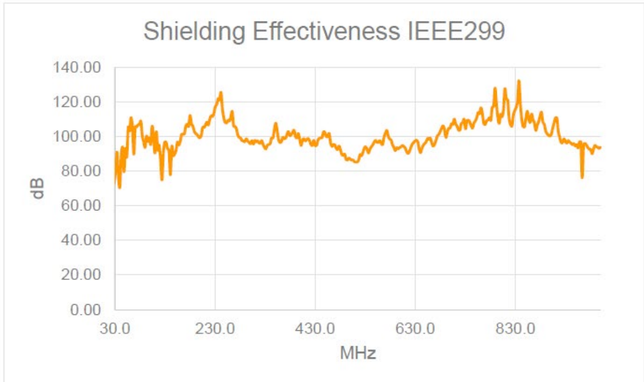
Test Position 6, 30 - 1000 MHz Vertical
