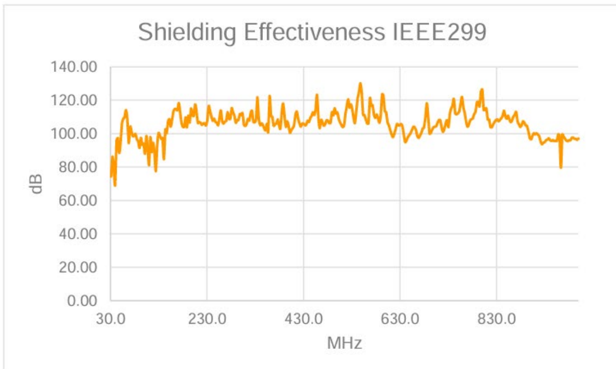
Test Position 11, 30 - 1000 MHz Vertical
