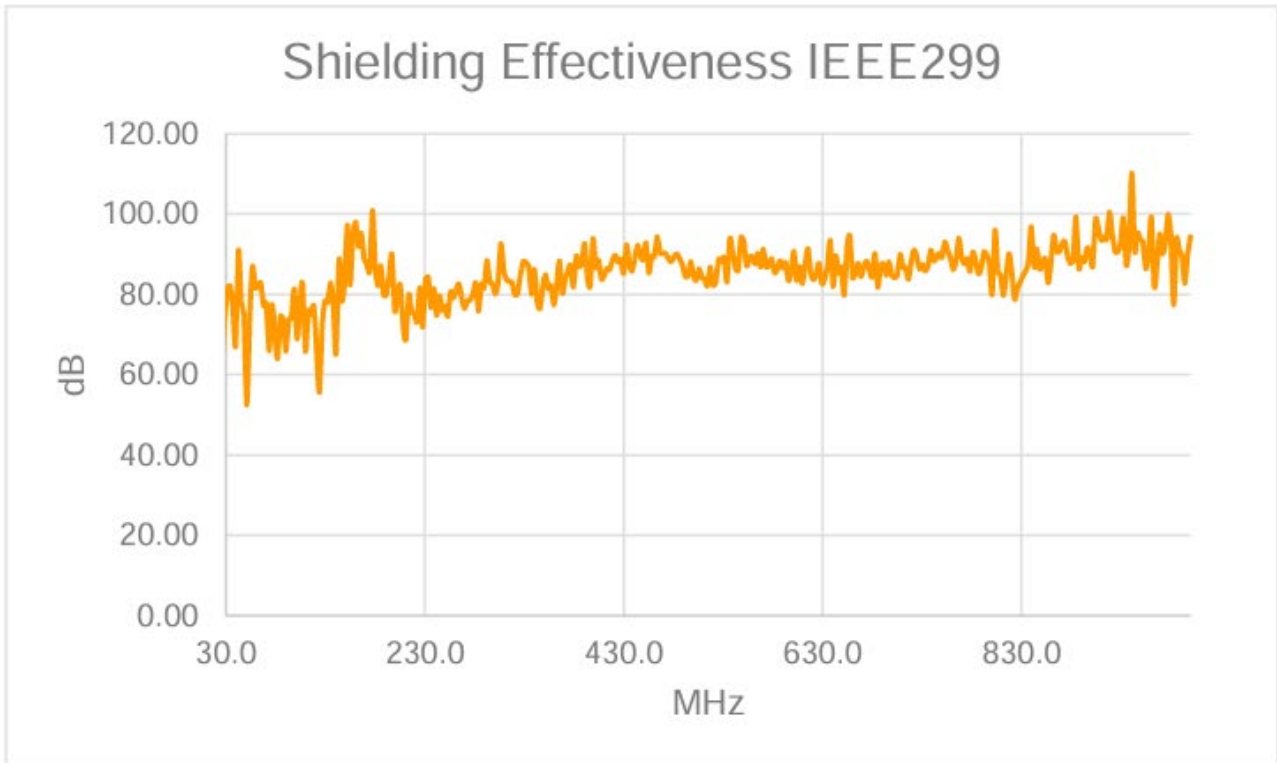
Test Position 8, 30-1000 MHz Vertical
