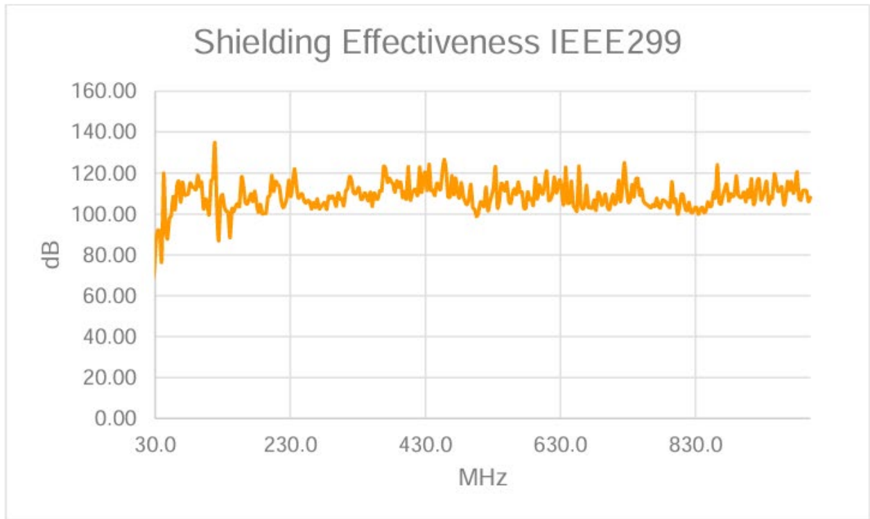
Test Position 19, 30 - 1000 MHz Vertical
